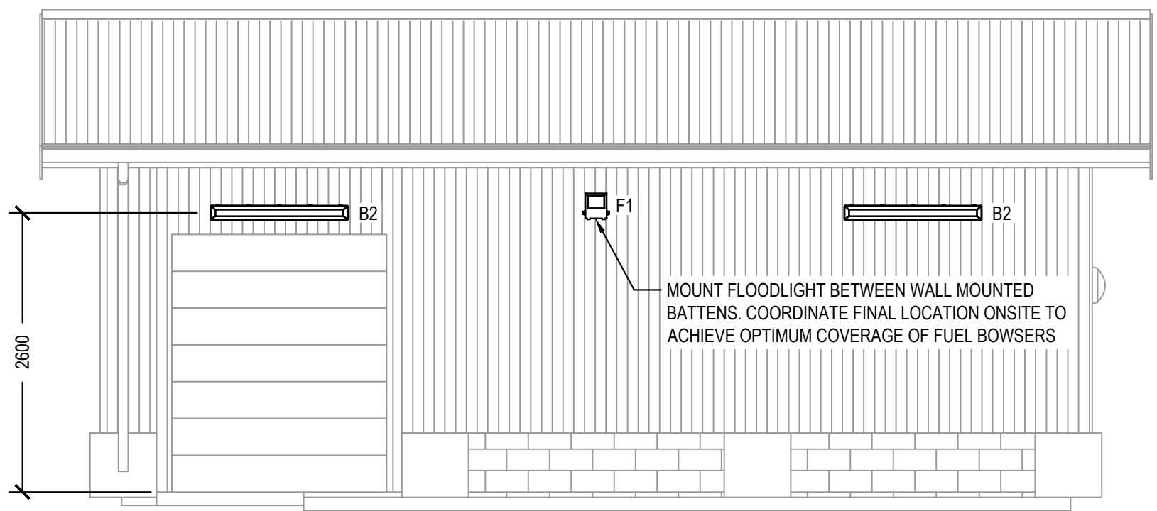
ELEVATION PLAN 1:50
